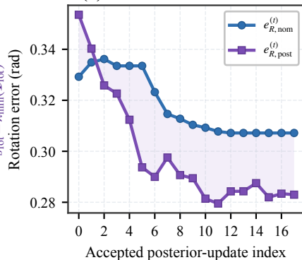
(b) Rotational error evolution
